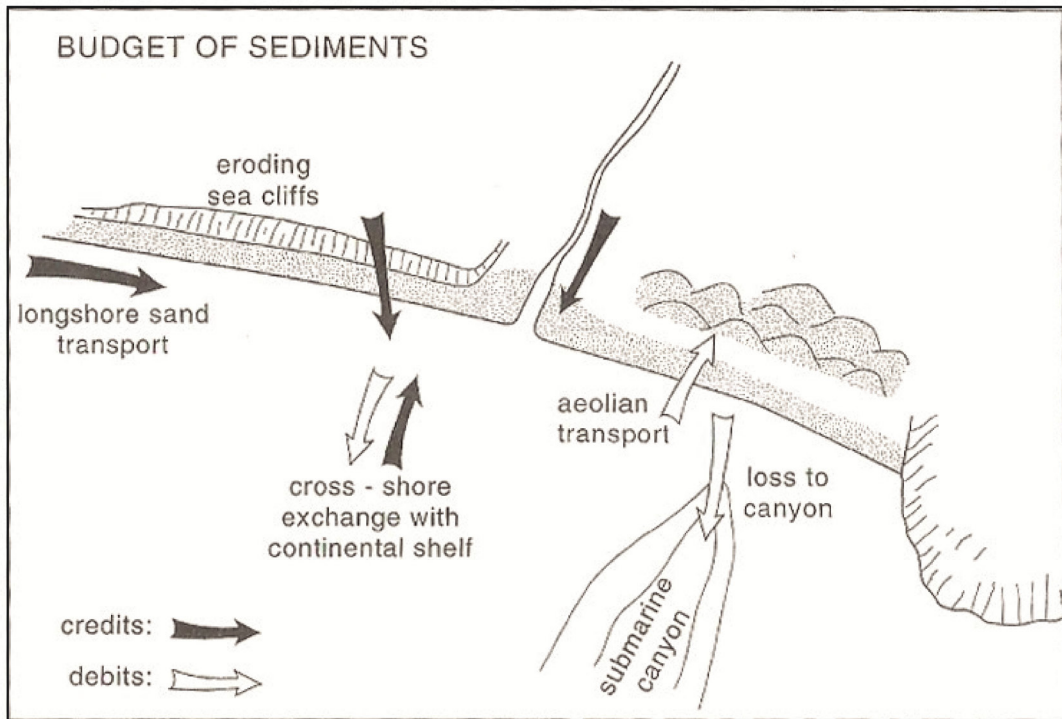
FIG. 2. Schematic diagram of the concept of a littoral cell and its main components. After Komar (1998).
