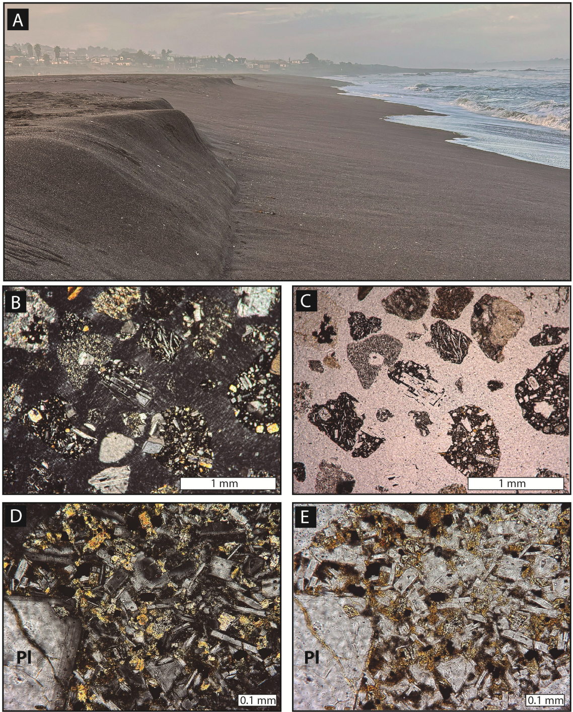
FIG. 4. Pichilemu sand sample. A. View toward the south of Playa La Ballena, showing the sand bank from which samples were collected for petrographic examination. B-C. Cross-polarized and plane-polarized photomicrographs showing representative volcanic sand grains mounted in resin. D-E. Cross-polarized and plane-polarized photomicrographs showing a sand grain with smectite as an alteration product of volcanic glass occurring interstitially within the groundmass.
