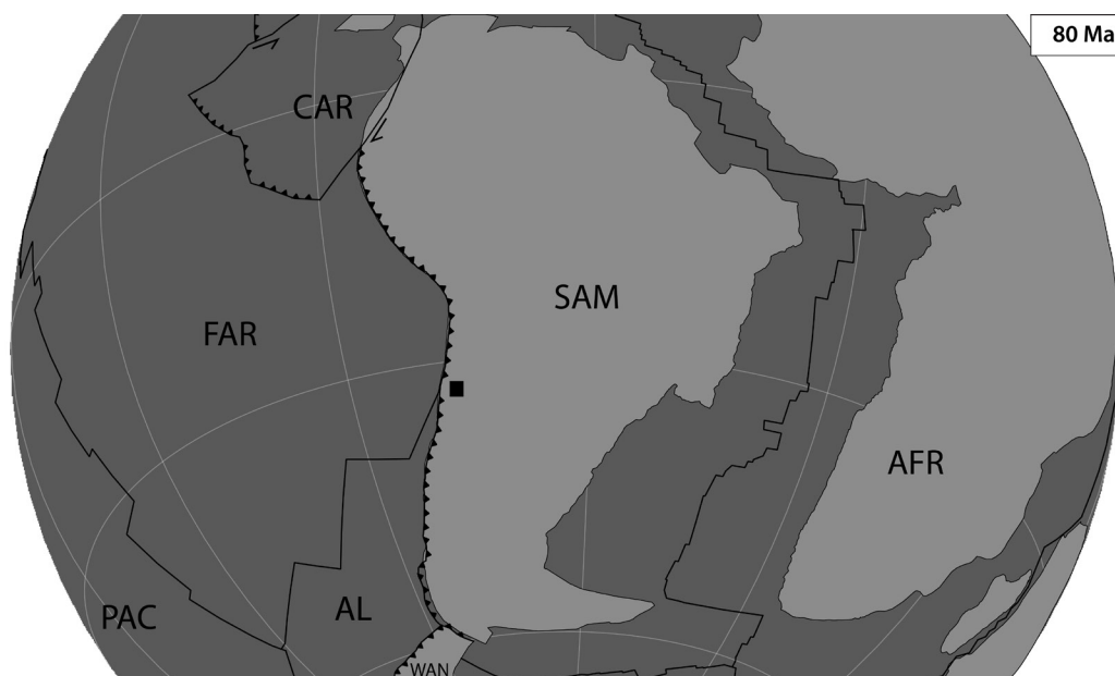
FIG. 12. Tectonic plate reconstruction at ~80 Ma for South America according to Müller et al. (2019). The black square shows the location of the study area. SAM : South American plate; FAR : Farallon plate; AL : Aluk plate; PAC : Pacific plate; CAR : Caribbean plate; AFR : African plate; WAN : West Antarctic plate.
