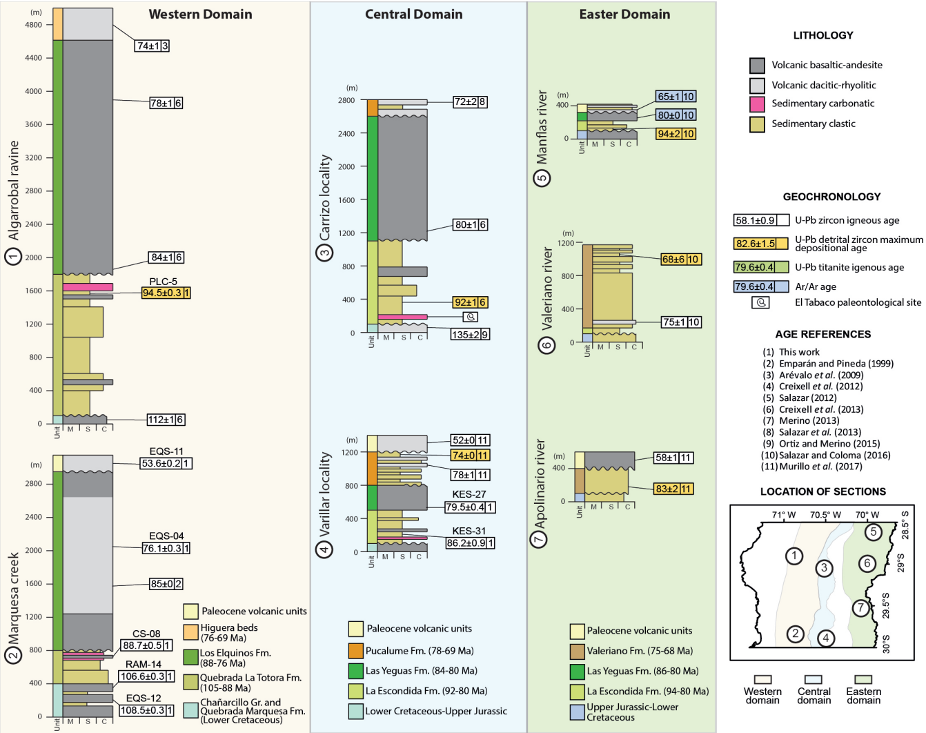
FIG. 5. Synthetic stratigraphic columns for Cretaceous units in the three stratigraphic domains defined in this study. Column thicknesses in meters. See figures 2 and 3 for comparisons and spatial context. M=Mudstone; S=Sandstone; C=Conglomerate.
