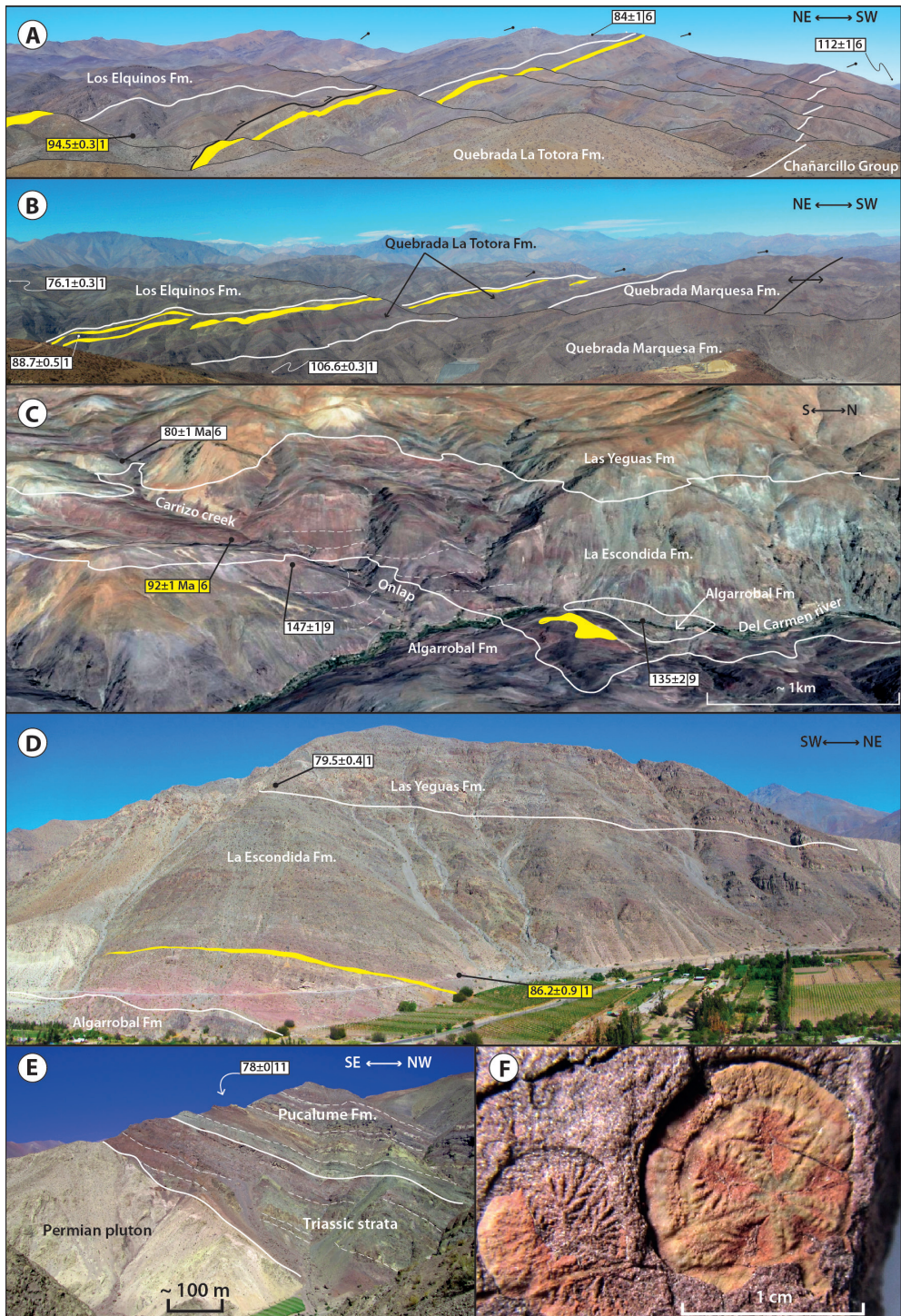
FIG. 6. Field photographs of key stratigraphic features from Cretaceous units along the study area. A. Western Domain, Algarrobal ravine area. Thick black line with arrows shows reverse fault. B. Western Domain, Marquesa creek area. C. Central Domain, El Carrizo locality, where the La Escondida Formation onlaps onto the eroded Algarrobal Formation. D. Central Domain, Varillar locality. E. Central Domain, north of Varillar locality. F. Central Domain SNGM-2032 Isselicerinus? sp. fossils from the La Escondida Formation. Yellow swaths enclose carbonate strata. Thick, solid white lines show stratigraphic contacts. Thin, segmented white lines show stratification. Age references same as in figures 3 and 5. Panel C from Google Earth.
