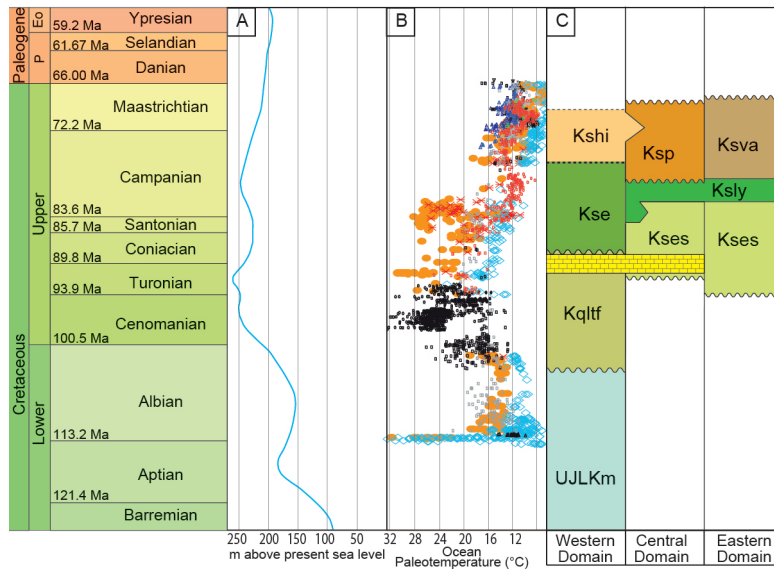
FIG. 10. Comparison of global oceanic events with local stratigraphy for the Aptian-Thetanian. A. Global eustatic curve after Haq (2014). B. Ocean paleotemperature data from isotopic analysis of benthic and planktonic foraminifers compiled by Friedrich et al. (2012) and Huber et al. (2018). Black squares and triangles: North Atlantic (benthic). Gray squares: Southern high latitudes (benthic). Red squares: Pacific Ocean (benthic). Blue triangles: Subtropical South Atlantic (benthic). Green squares: Indian Ocean (benthic). Orange circles: South Atlantic and South Indian oceans (planktonic). Light blue diamonds: South Atlantic and South Indian oceans (benthic). Red asterisks: South Atlantic and South Indian oceans (deep planktonic). C. Local stratigraphy from this study, as in figure 7. Yellow band shows carbonate intervals in the Western and Central domains.
