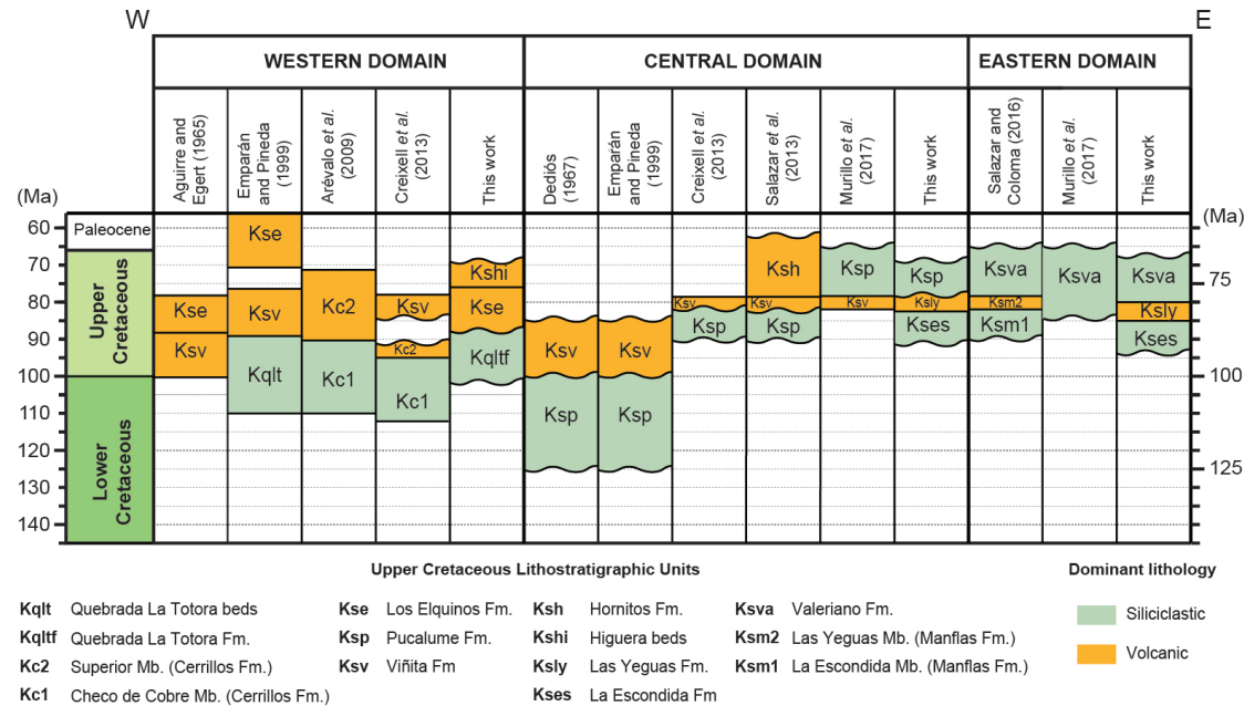
FIG. 2. Summary of Upper Cretaceous stratigraphic nomenclature available in the literature for the 28.5-30° S segment.
