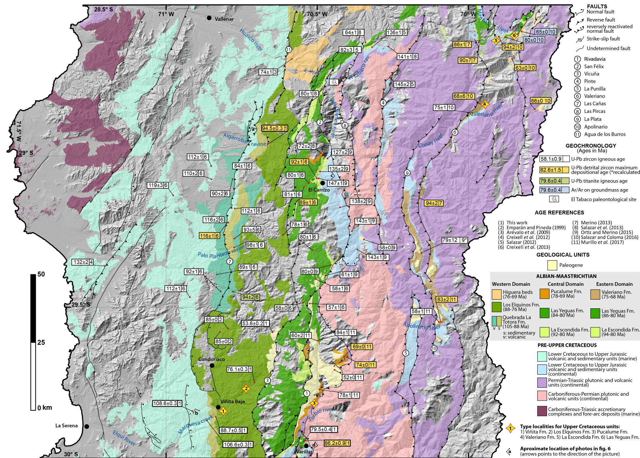
FIG. 3. Geological map of the study area, showing stratified Cretaceous rocks. Black circles refer to main towns and cities. Former Quebrada La Totorá beds and La Escondida and Las Yeguas members are referred to as formations after this work (see text for more details). All ages are listed in Supplementary Table 1.
