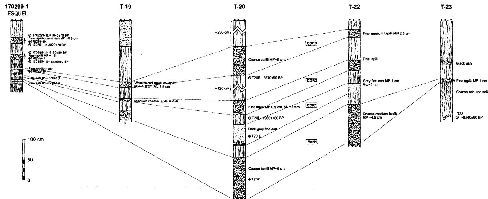
FIG. 4. Diagram showing the correlation of different tephra deposits occurring in the soil profiles located in figure 2. These correlations were based on the internal characteristics of the tephra, their age (Table 1) and chemical composition (Table 2 and Fig. 3). Maximum pumice size (MP) and scoria size (MS) are indicated.
