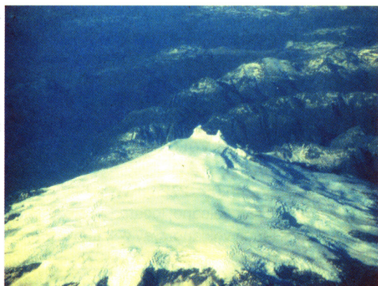
FIG. 11. Photograph of the small ice-filled summit crater of the Melimoyu volcano looking east.
