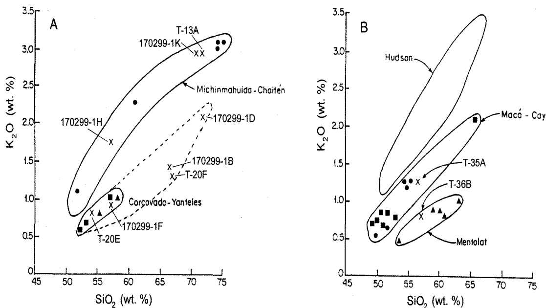
FIG. 3. \text{SiO}_2 versus \text{K}_2\text{O} of pumice collected from tephra fall deposits compared to the range of composition of samples from different volcanic centers in the region 42^\circ 30' to 45^\circ\text{S} . Fields for Michinmahuida/Chaitén (circles) are from López-Escobar et al. (1993) and Stern et al. (2002), for Corcovado (squares) and Yanteles (triangles) from López-Escobar et al. (1993), for Macá (circles) and Cay (squares) from Futa and Stern (1988) and López-Escobar et al. (1993), and for Mentolat (triangles) from López-Escobar et al. (1993).
