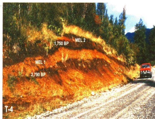
FIG. 12. Photograph (CS-1) at site T-4 (Fig. 2), a road cut along the Carretera Austral 22 km north of the town of Puyuhuapi, showing the two late Holocene tephra deposits derived from explosive eruptions of the Melimoyu volcano. The older deposit MEL1 is compositionally layered, grading upwards from white dacitic pumice into very dark mafic scoria, almost as dark as the organic-rich soils which contain the tephra layers.
