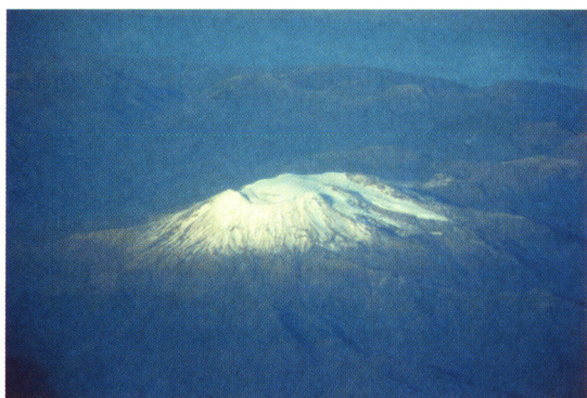
FIG. 13. Photograph of the dome and/or ice filled summit caldera of the Mentolat volcano as seen from the west.
