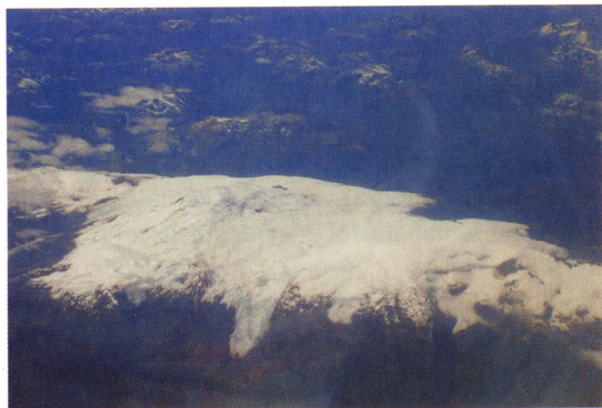
FIG. 7. Photograph of the ice covered Michinmahuida volcano as seen from the west.
