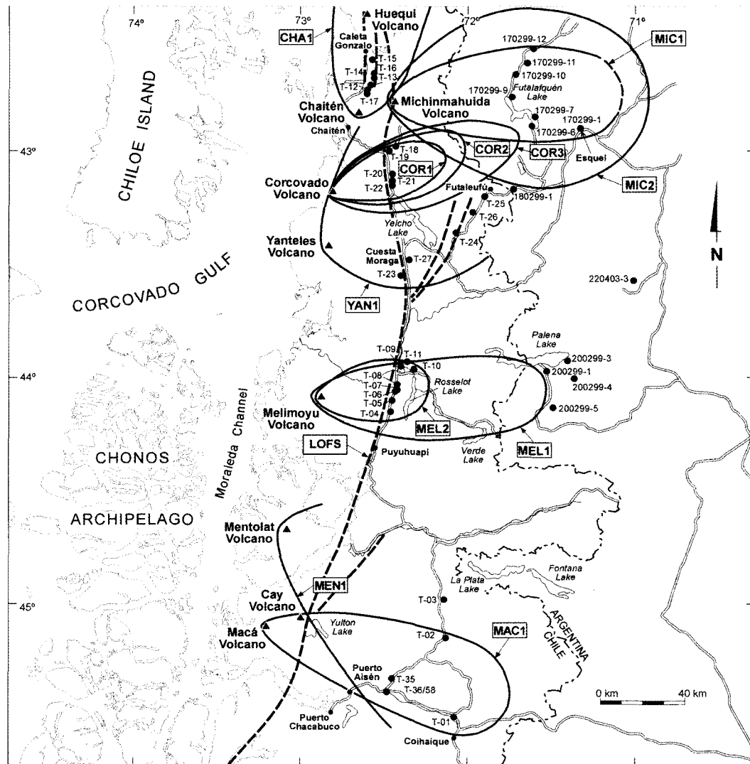
FIG. 2. Map showing the location of volcanoes and road-cut sites studied between 42°30' and 45°S, as described in the text, and the approximately 10 cm isopachs of the eleven Holocene eruptions identified in this area. LOFS = Liquiñe-Ofqui Fault System.
