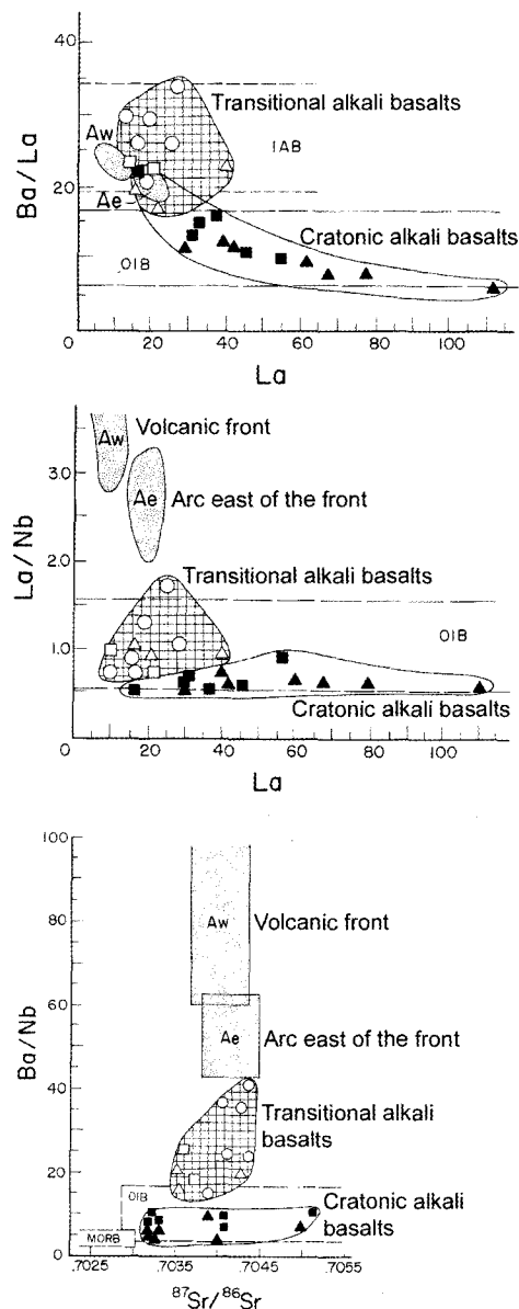
FIG. 8. A. Ba/La versus La content; B. La/Nb versus La content; and C. Ba/Nb versus ^{87}Sr/^{86}Sr , for samples from along the volcanic front (Aw) of the Central SVZ, CSVZ centers east of the front (Ae), and back-arc alkali basalts in areas of Cenozoic arc volcanism (transitional alkali basalts, open circles and triangles; Stern et al. , 1990) and cratonic regions that have not experienced Cenozoic arc volcanism (cratonic alkali basalts; solid squares and triangle; Stern et al. , 1990). Figure 8 illustrates the higher Ba/La , La/Nb and Ba/Nb ratios, and La contents, from west to east across the CSVZ arc and into the back-arc region, interpreted to result from decreasing influx of slab-derived fluids into the subarc asthenospheric mantle wedge, and, as a consequence, decreasing degree of partial mantle melting across the arc.
