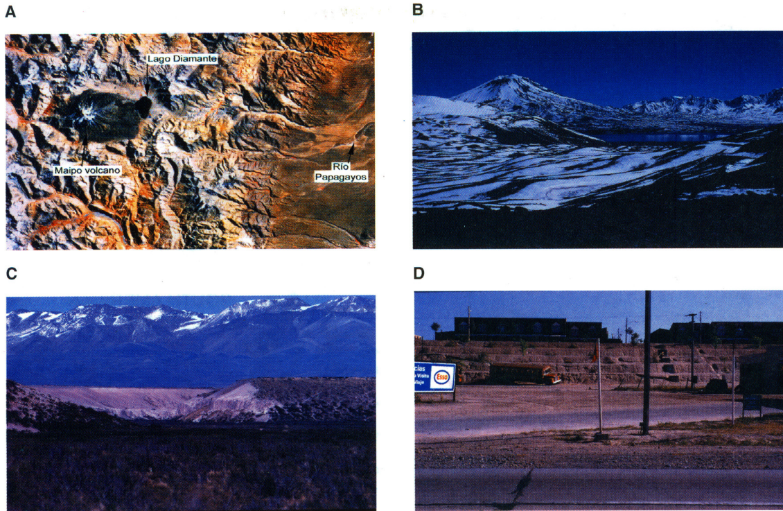
FIG. 5. A. Satellite photo of the Maipo volcano and Diamante lake inside the elliptical 15 by 20 km Diamante caldera. B. The Maipo volcano and Diamante lake inside the Diamante caldera wall. C. Partially welded rhyolite tuffs, derived from the Pleistocene eruption of the Diamante caldera, which outcrop along the Papagayos river in Argentina. D. The 30 m thick Tuff of Pudahuel, also derived from the Pleistocene eruption of the Diamante caldera, outcropping along the road to the international airport west of Santiago, Chile. The Diamante caldera formed at 450 \pm 60 ka, and the volume of rhyolite tuff erupted in this event is estimated as approximately 450 \text{ km}^3 (Stern et al. , 1984a).
