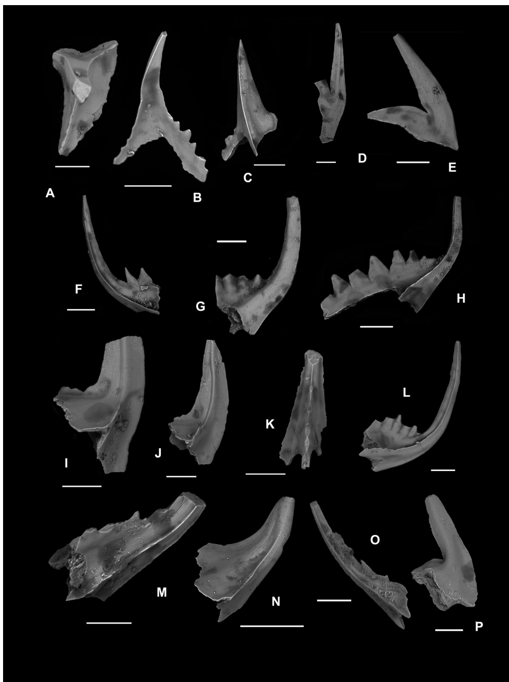
FIG. 3. Dapingian conodonts from the Huaytiquina section, Baltoniodus navis Zone. SEM Microphotographs. A-H. Baltoniodus cf. B. navis (Lindström). A, B. Pa element, upper view and anterior view respectively, sample H5, CML-C 3500(1), 3501(1). C. sinistral Pb element, anterior-lateral view, sample H5, CML-C 3502(1). D, E. M elements, lateral views, sample H5, CML-C 3507(1,2). F. Sa element, lateral view, sample H5, CML-C 3503(1). G. Sc element, lateral view, sample H5, 3505(1). H. Sd element, lateral view, sample H5, CML-C 3506(1). I-M. Gothodus cf. G. costulatus Lindström. I. Pa element, lateral view, sample HA, CML-C 3508(1). J. Pb element, lateral view, sample HA, CML-C 3509(1). K. Sa element, lateral view, sample HA, CML-C 3510(1). L. Sb element, lateral view, sample HA, CML-C 3511(1). M. Sd element, lateral view, sample HA, CML-C 3513(1). N-P. Trapezognathus quadrangulum Lindström. N. Pb element, lateral view, sample H5, CML-C 3515(1, 2). O. Sa element, lateral view, Sample H5, CML-C 3516(1, 2). P. M element, lateral view, sample H5, CML-C 3517(1). Scale bars: 0,1 mm.
