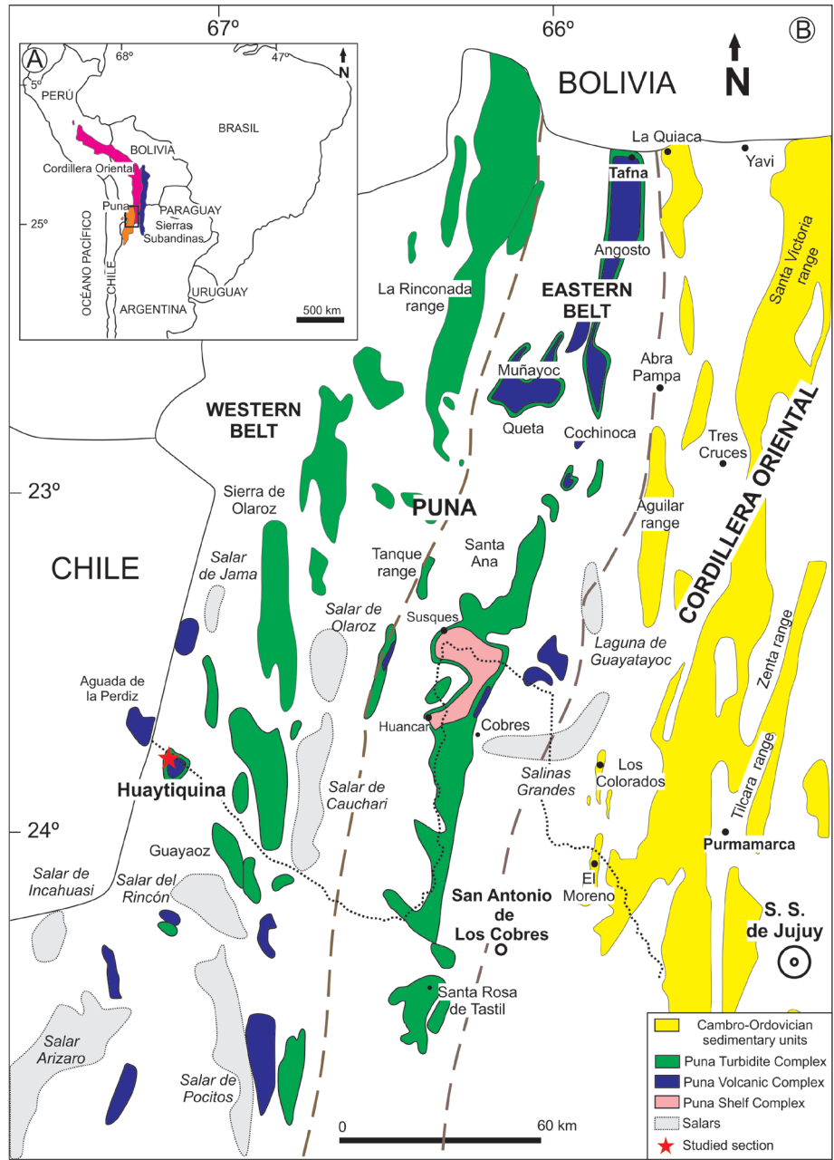
FIG. 1. Location map of northwestern Argentina showing the Ordovician deposits and fossiliferous localities at the Argentine Puna region and the Cordillera Oriental.
