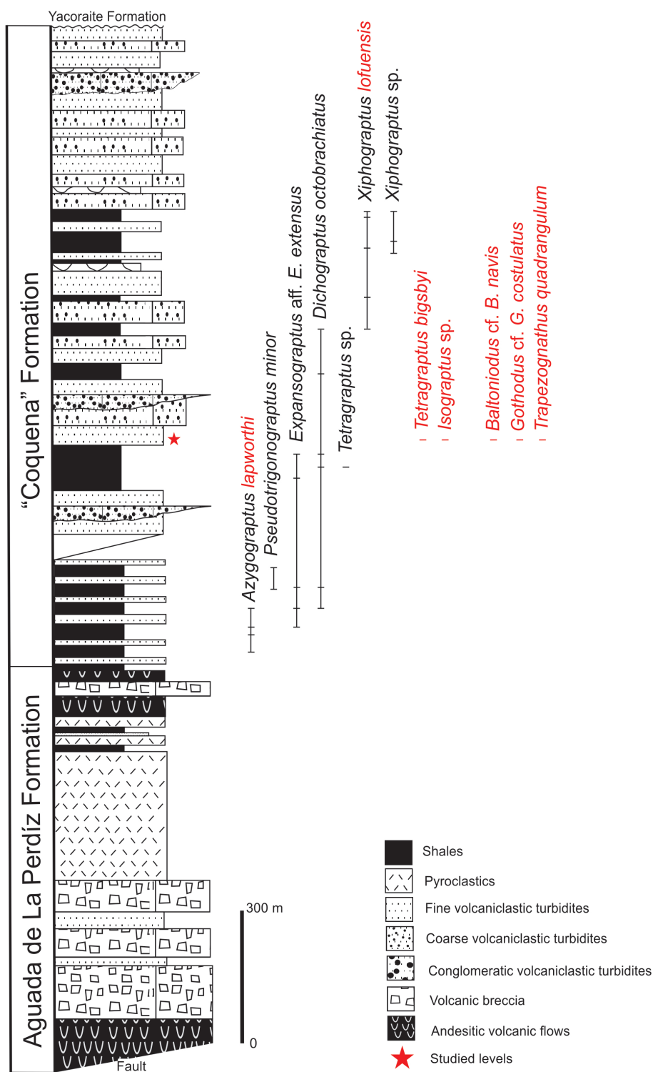
FIG. 2. Stratigraphic column of the Huaytiquina section at western flank of the Argentine Puna (modified in red from Monteros et al. , 1996: fig. 2), displaying the stratigraphic ranges of the significant graptolite and conodont taxa.
