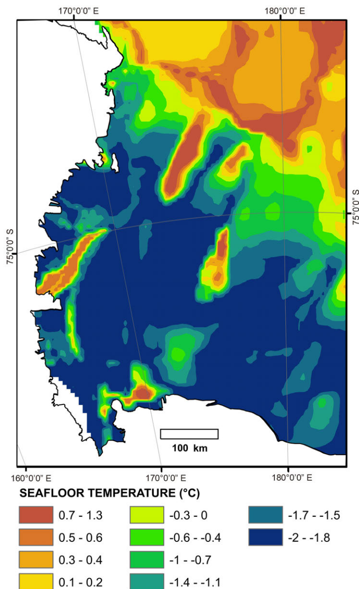
FIG. 2. Seafloor temperature distribution (in degrees celsius), water column temperature data from National Oceanographic Data Center website.
