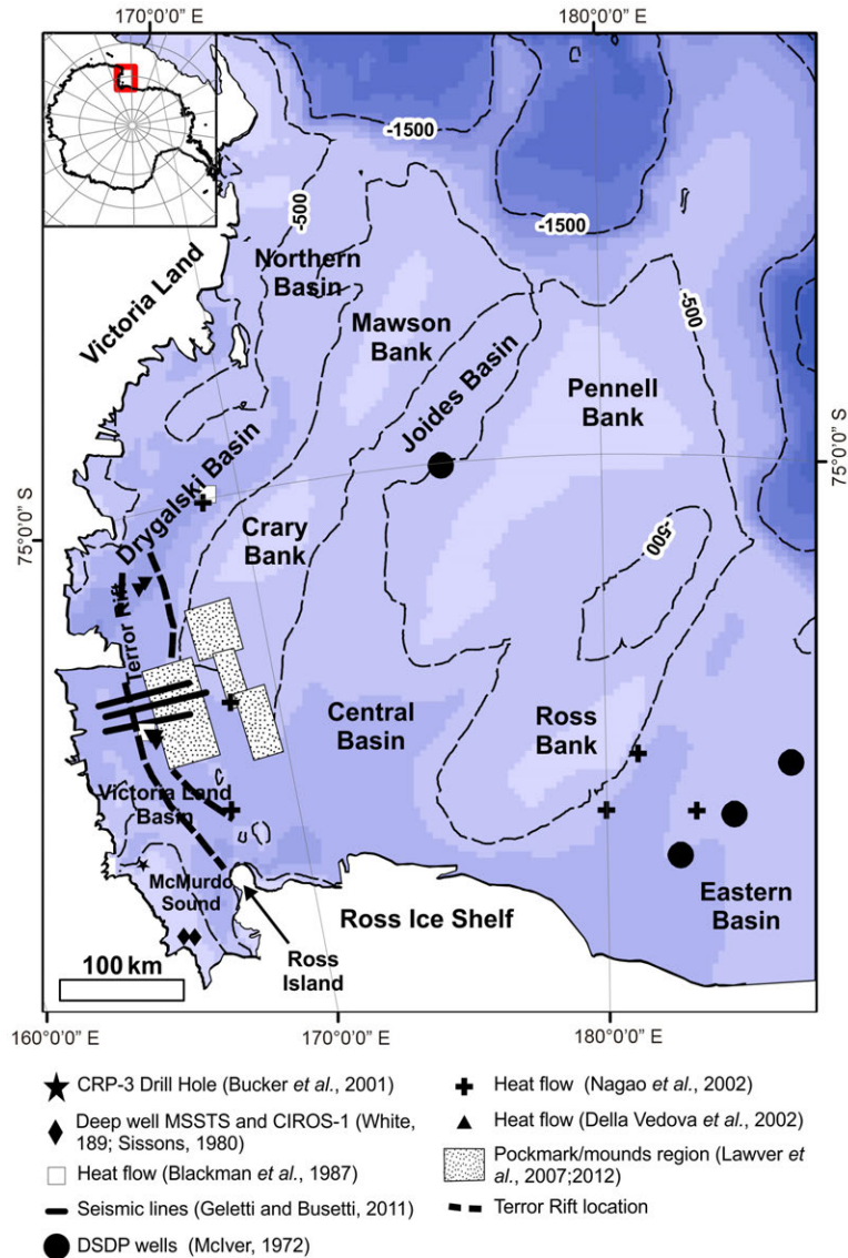
FIG. 1. Map of the study area including bathymetry in meters. Position of multichannel seismic data, heat flow measurements and pockmark/mound region are showed. See details in the text.
