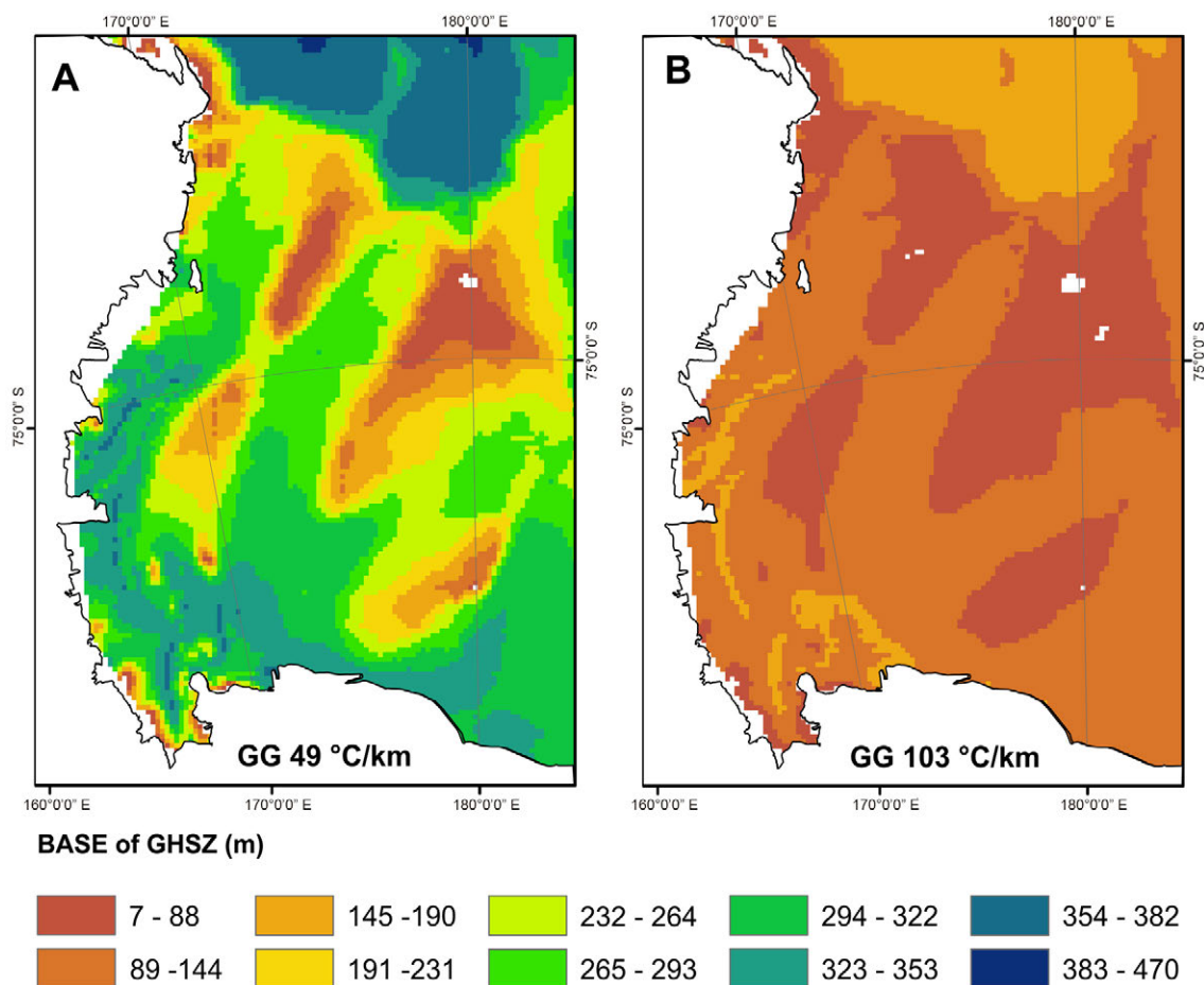
FIG. 3. Distribution of the base of the GHSZ from the seafloor (in meters). A. GG equal to 49 °C/km; B. GG equal to 103 °C/km.
