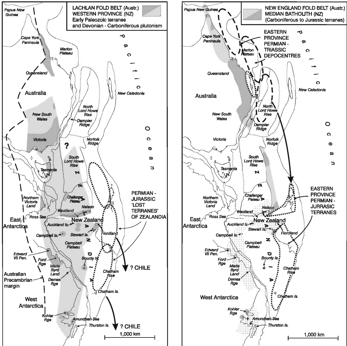
FIG. 1. The Pacific margin of Gondwanaland in a Late Triassic reconstruction showing: left diagram: late Neoproterozoic-early Paleozoic basement outcrop (dark grey shading) and possible geographic continuations (light grey shading) and the Precambrian craton margin (bold broken line). The bold dotted ellipses represent probable areas of late Paleozoic-Mesozoic sediment depocentres, that might now form lost terranes of Zealandia, destined for Chile (suggested tectonic transport direction shown as bold arrows); right diagram: late Paleozoic-Mesozoic outcrop (dark grey shading) and possible geographic continuations (light grey shading). Areas of Jurassic-Cretaceous plutonism are shown as stipple. The bold dashed ellipses represent probable areas of late Paleozoic-Mesozoic sediment depocentres that now form suspect terranes in the Eastern Province, New Zealand (bold dotted envelopes).
