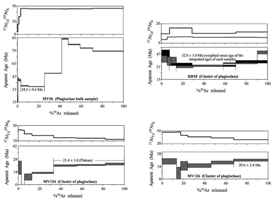
FIG. 4. ^{40}\text{Ar}/^{39}\text{Ar} and ^{37}\text{Ar}/^{39}\text{Ar}_{\text{Ca}} ratio spectra obtained on plagioclase bulk samples from the studied area for samples (a) MV56; (b) RB18; (c) MV154 y (d) MV126.
