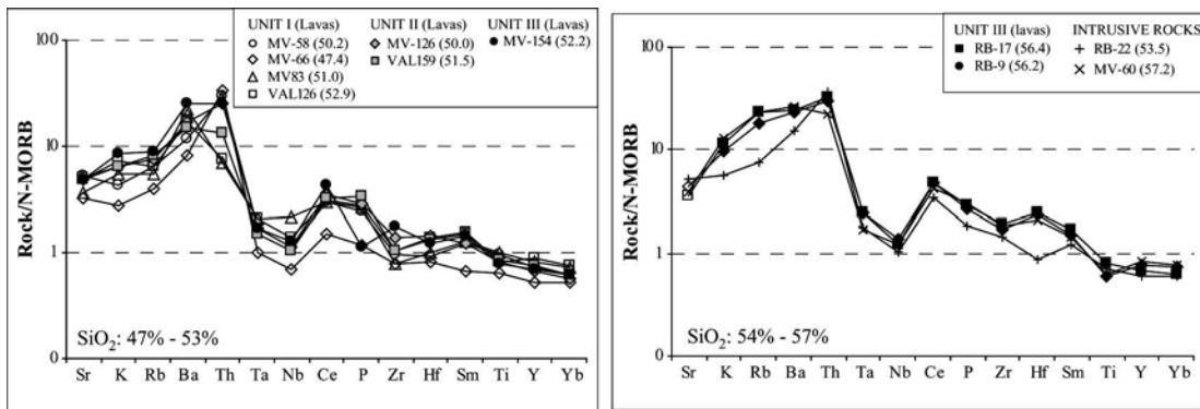
FIG. 10. N-MORB-normalized trace element diagrams for the samples from the studied area. Samples are plotted by rock type. SiO_2 contents (wt%) of the samples in parentheses. Normalizing values from Pearce (1983).
