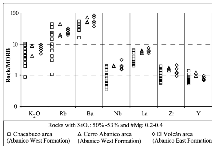
FIG. 14. Normalized concentrations for some trace element of the three compared localities. Normalizing values from Pearce and Parkinson (1993).
