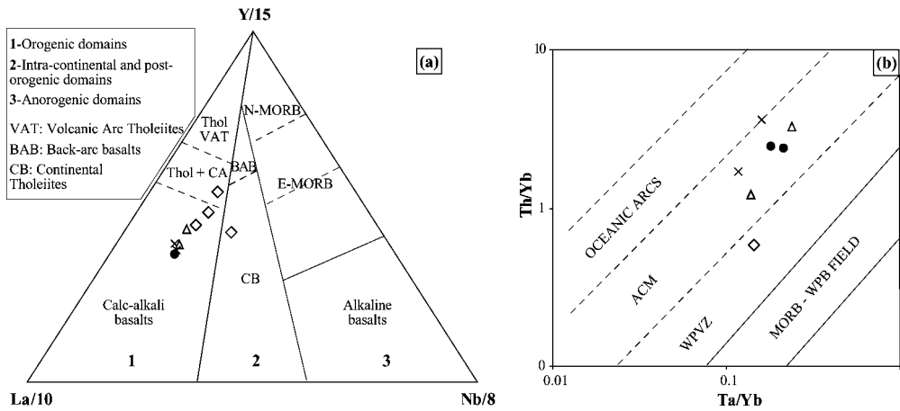
FIG. 11. Tectonic discrimination diagrams for (a) basic volcanic rocks (Cabanis and Lecolle, 1989) and (b) intermediate to acid volcanic rocks (fields taken from Gorton and Schandl, 2000). ACM- active continental margin; WPVZ- within plate volcanic zone; WPB- within plate basalts. Symbols as in figure 9.
