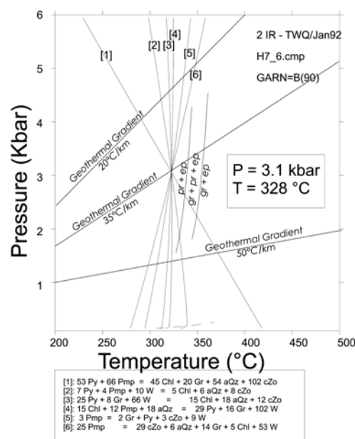
FIG. 6. P-T diagram in the CaO-MgO-Fe 2 O 3 -Al 2 O 3 -SiO 2 -H 2 O (CMFASH) system calculated using the GEO-CALC software (Berman et al. , 1987). Thermodynamic data base from Berman (1988) including solid-solution model of garnet from Berman (1990). Six multivariant reactions were modelled using pumpellyite (Pmp), hydrogarnet (Py and Gr), chlorite (Chl), epidote (cZo), quartz (aQz) and water (W). Reaction curves for the hydrogarnet (gr), prehnite (pr) and epidote (ep) from Liou et al. (1983).
